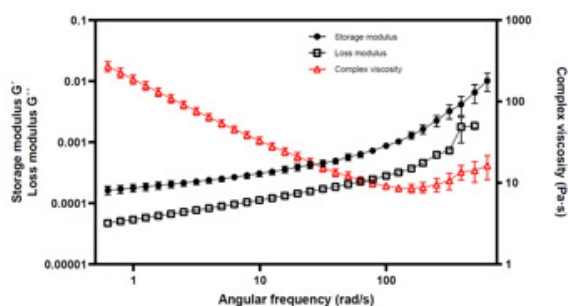
Fig. 1. Oscillation test.
